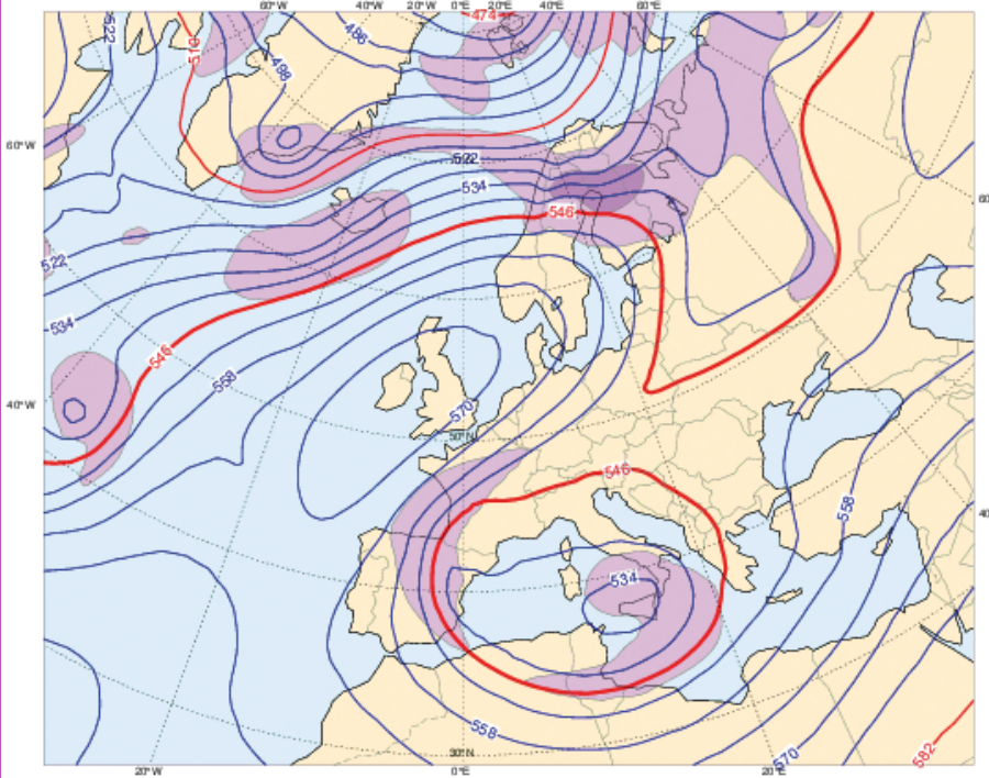
Mon 16 Jan 2017 00UTC @ECMWF Forecast T+96 VT: Fri 20 Jan 2017 00UTC 500hPa Geopotential High-Resolution Forecast, and Standard Deviation (shaded)
